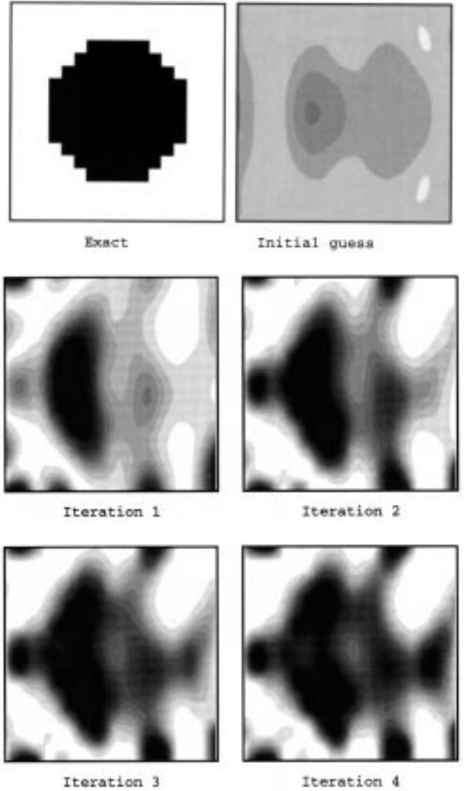
Fig. 4. Reconstruction of the characteristic function \chi versus iteration with the NK method for noisy data with a SNR of 30%.
