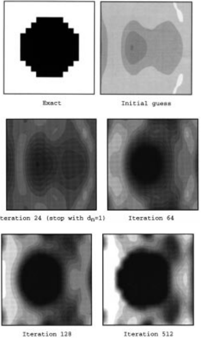
Fig. 7 Reconstruction of the characteristic function \chi versus iteration with the MG method for noiseless data. Only the update direction relative to \chi ( d_n ) is taken to be zero.
